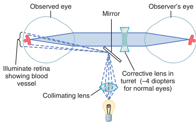
Figure 50-18. Optical system of the ophthalmoscope.
