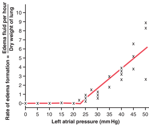
Figure 39-7. Rate of fluid loss into the lung tissues when the left atrial pressure (and pulmonary capillary pressure) is increased. (From Guyton AC, Lindsey AW: Effect of elevated left atrial pressure and decreased plasma protein concentration on the development of pulmonary edema . Circ Res 7:649, 1959.)
